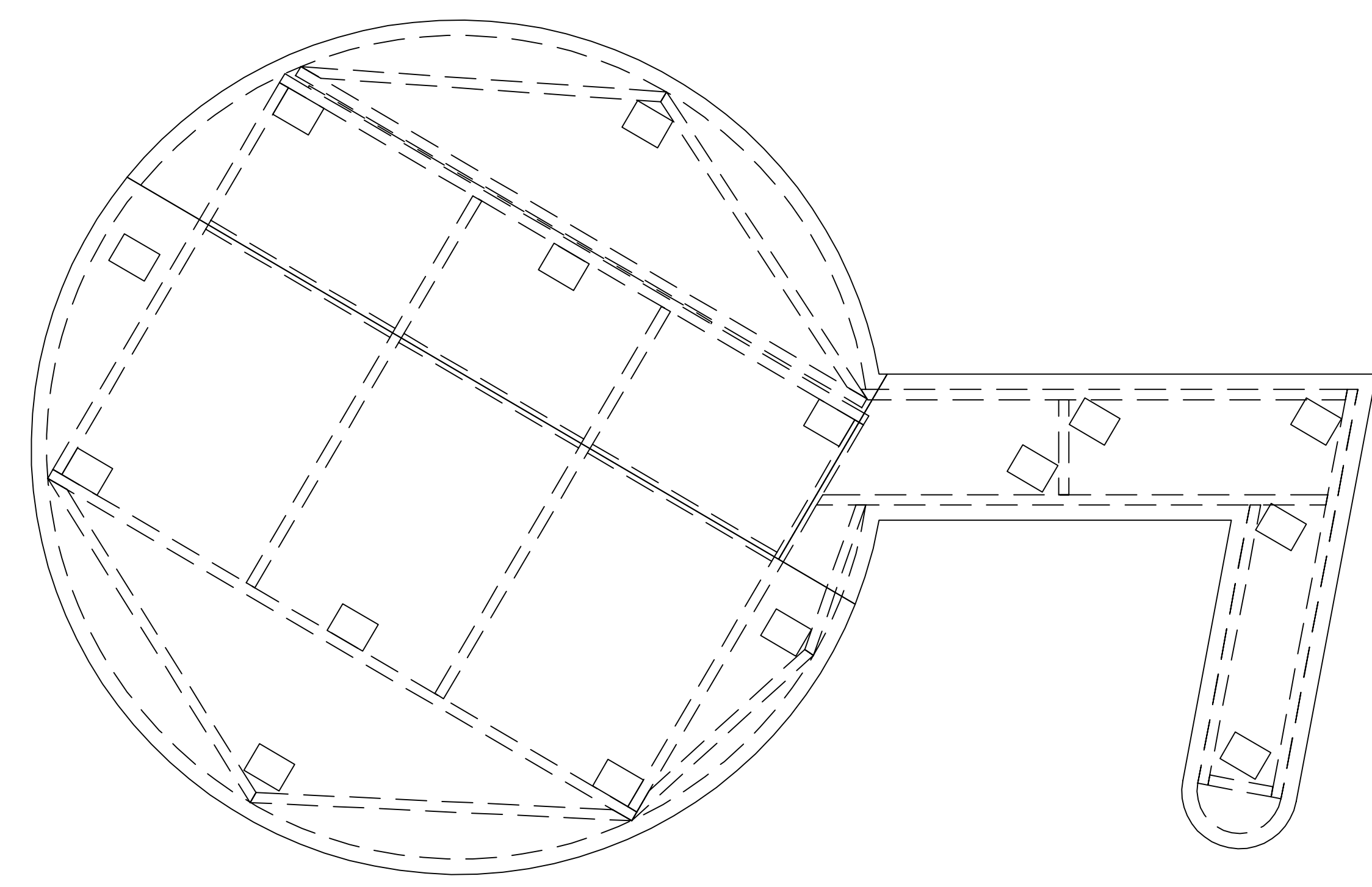
ALLEY WAGONS CASTER PLACEMENT
