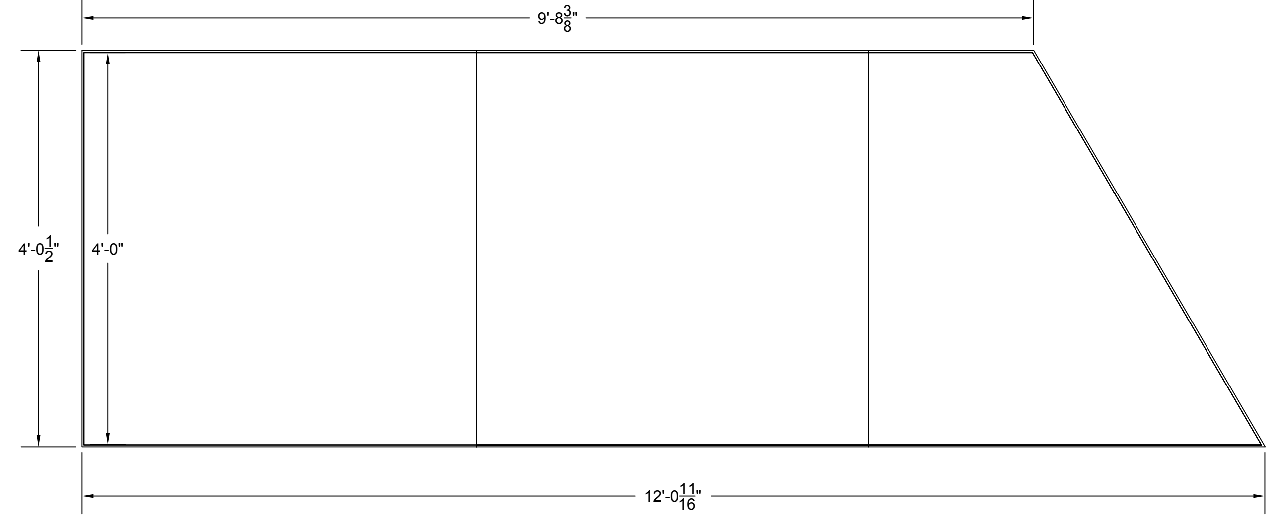
FRONT VIEW SIGN SIDE FLAT LAUAN
