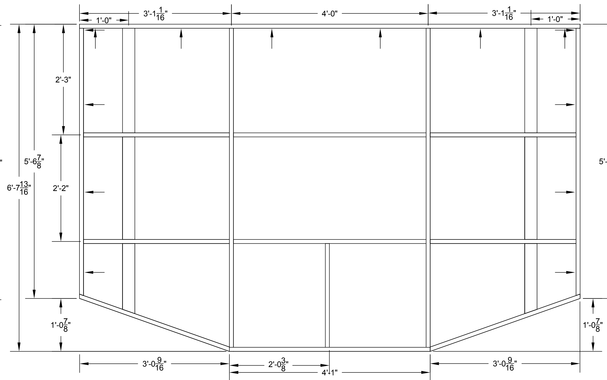
HOUSE WAGON FRAMING PLATFORM D
