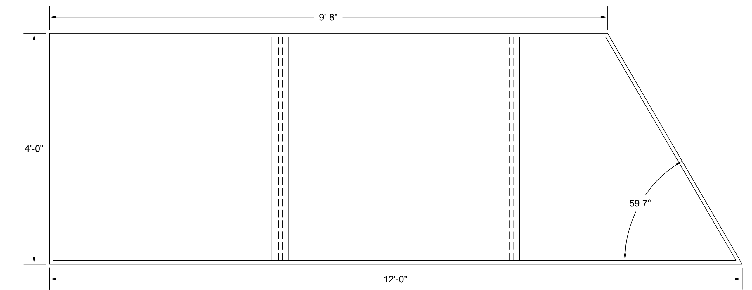
FRONT VIEW SIGN SIDE FLAT FRAMING
