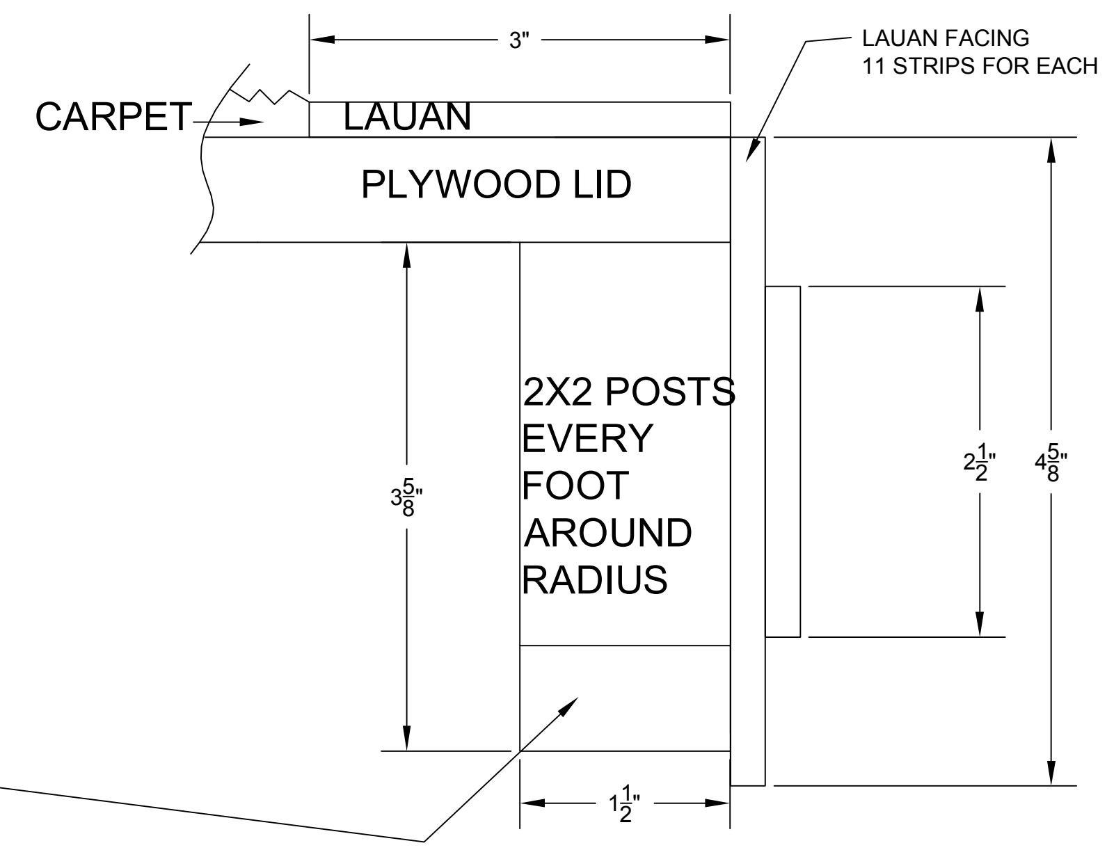
ALLEY WAGON FACING DETAIL FULL SCALE
