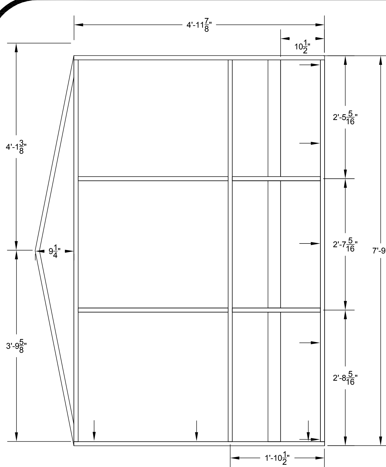
HOUSE WAGON FRAMING PLATFORM A
