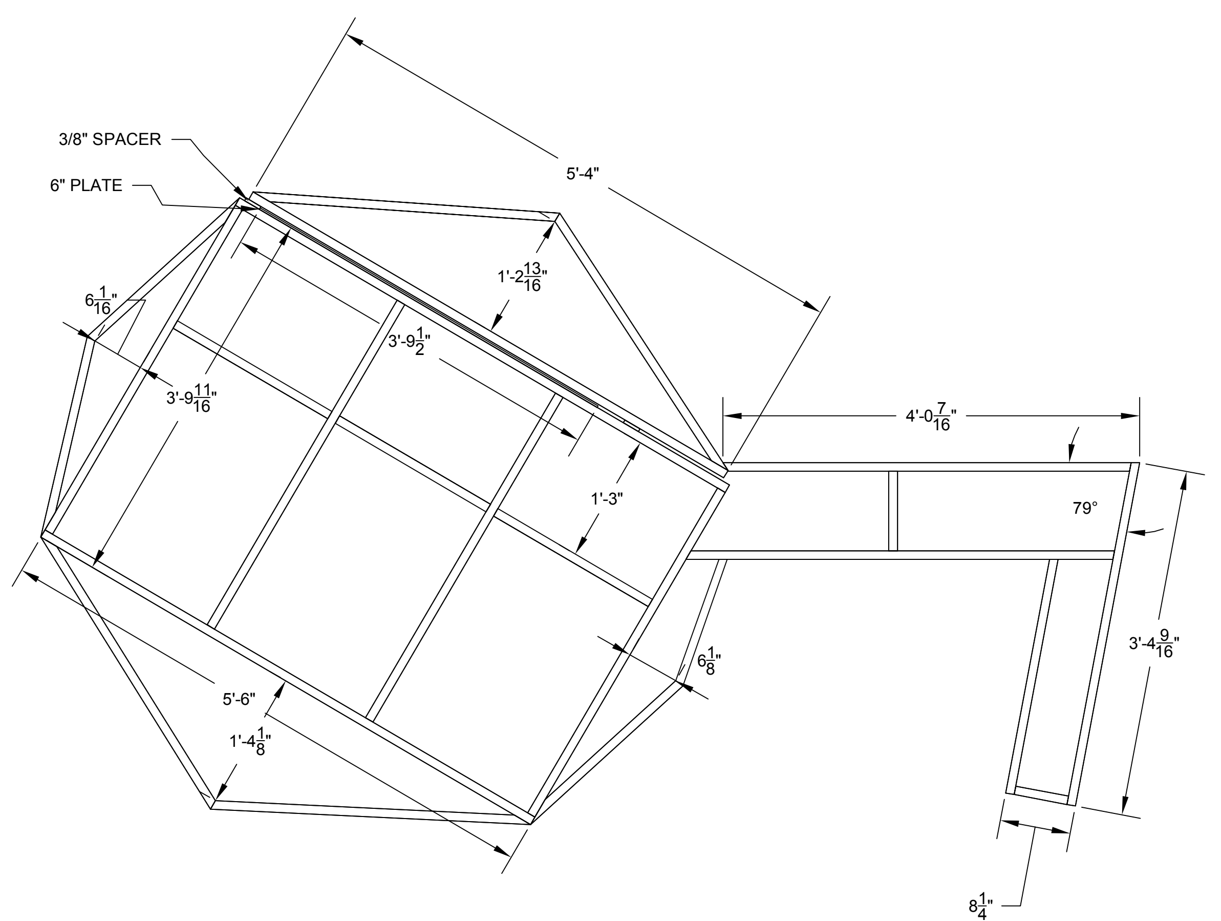
ALLEY WAGONS 1X3 FRAMING
