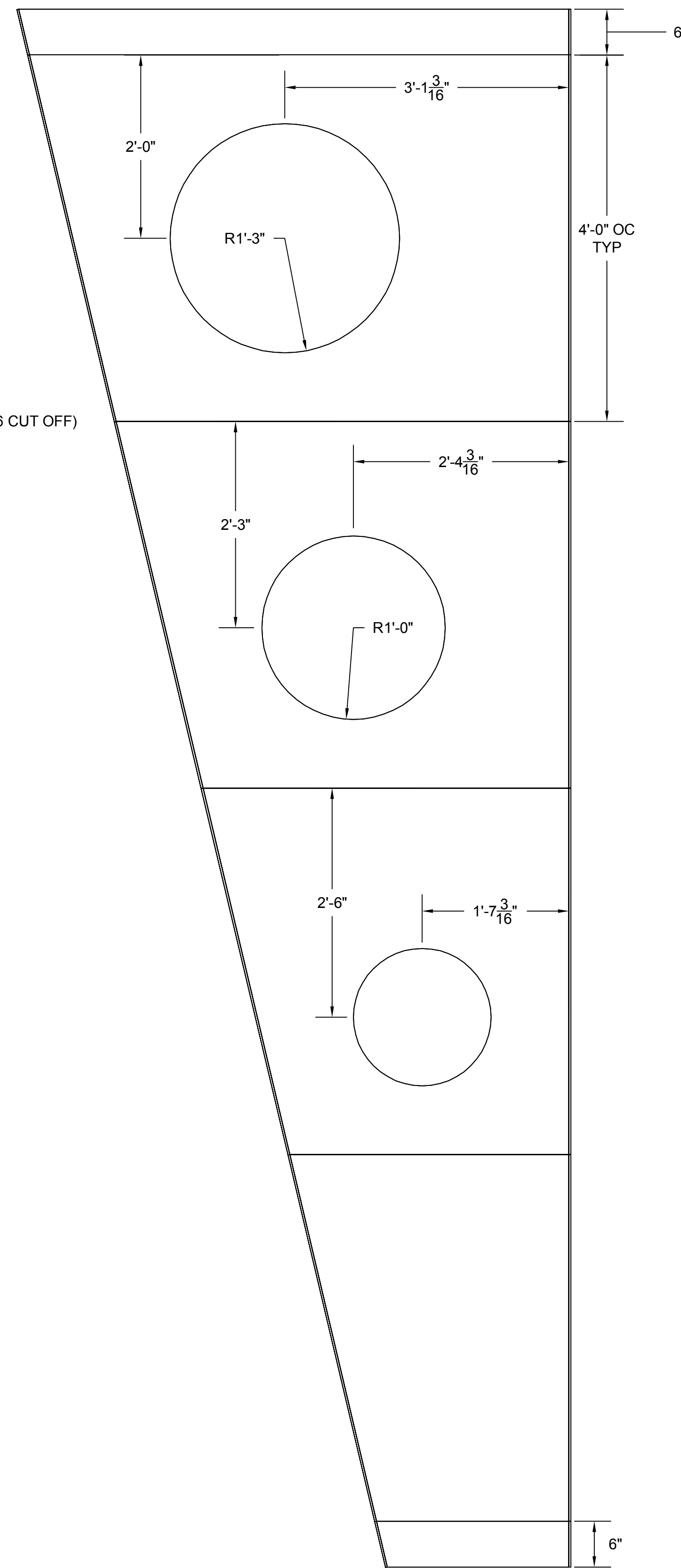
FRONT LAUAN SR UNIT
