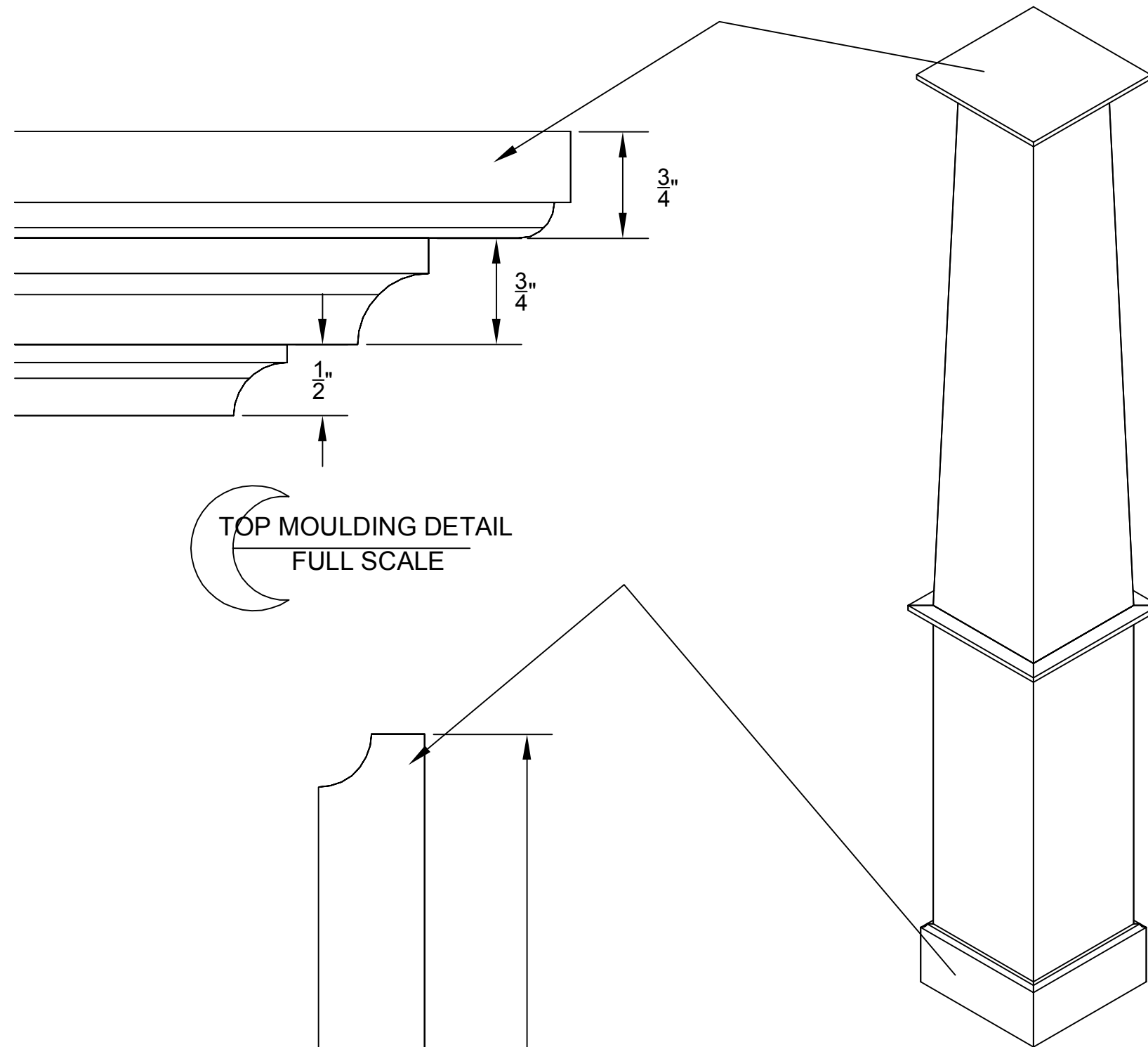
ASSEMBLED VIEW SCALE: 1"=1'-0"
