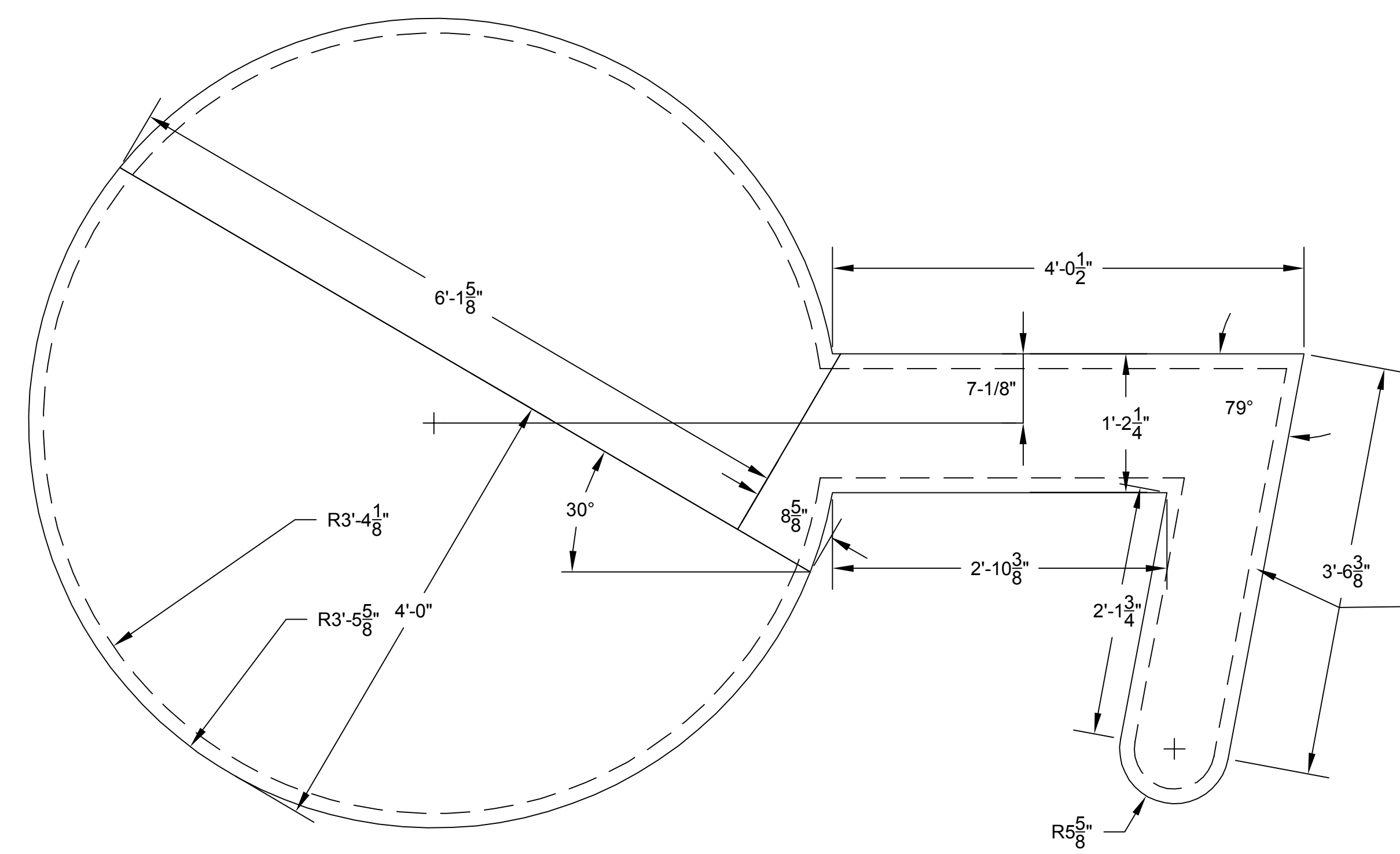
ALLEY WAGONS PLY AND PLY RIB LAYOUT
