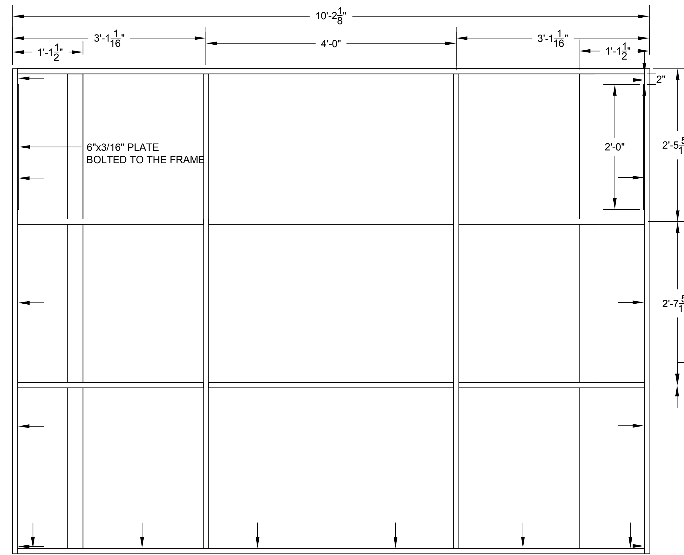
HOUSE WAGON FRAMING PLATFORM C
