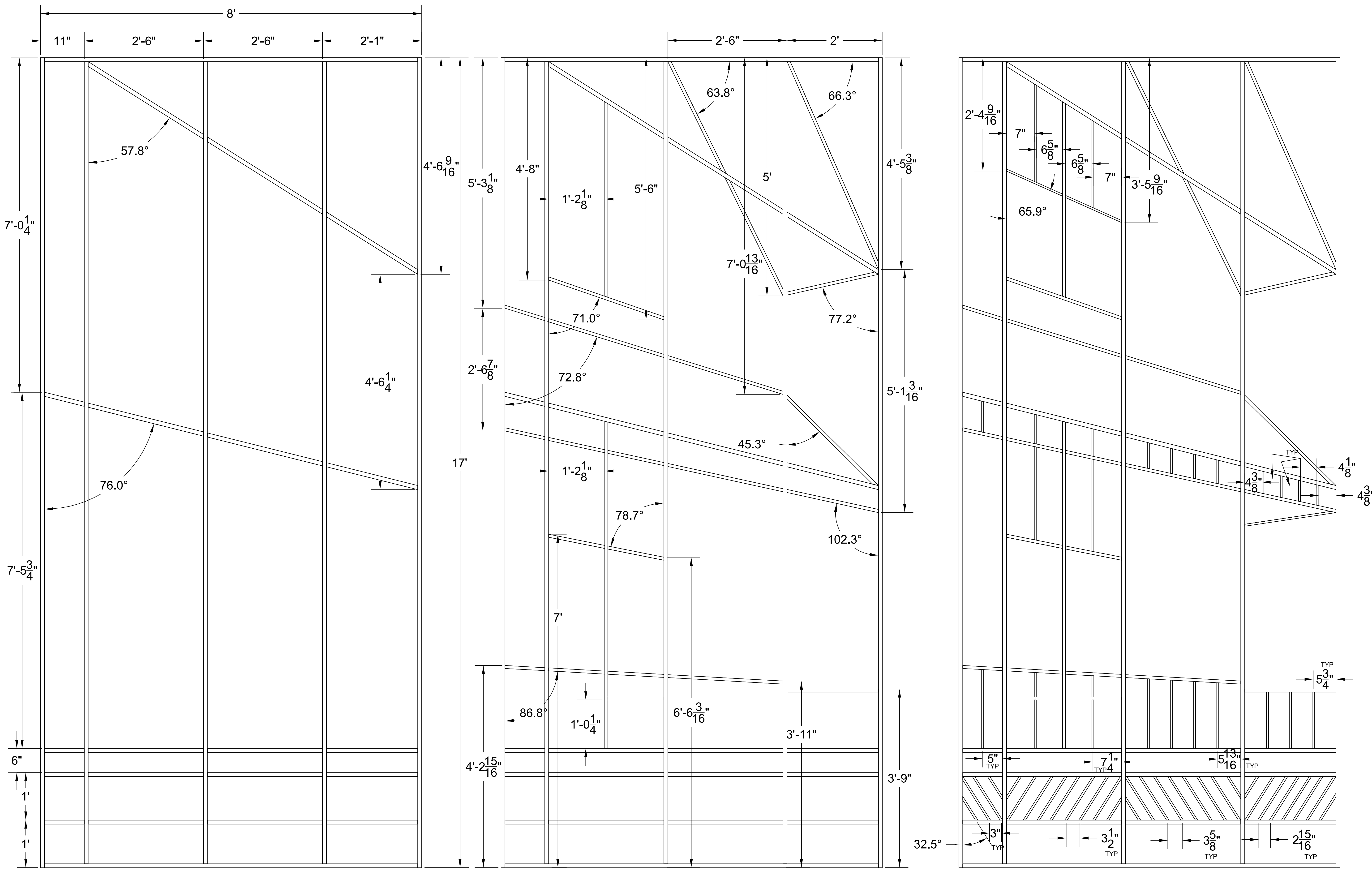
SR TRACKING PANEL 1" BOX
