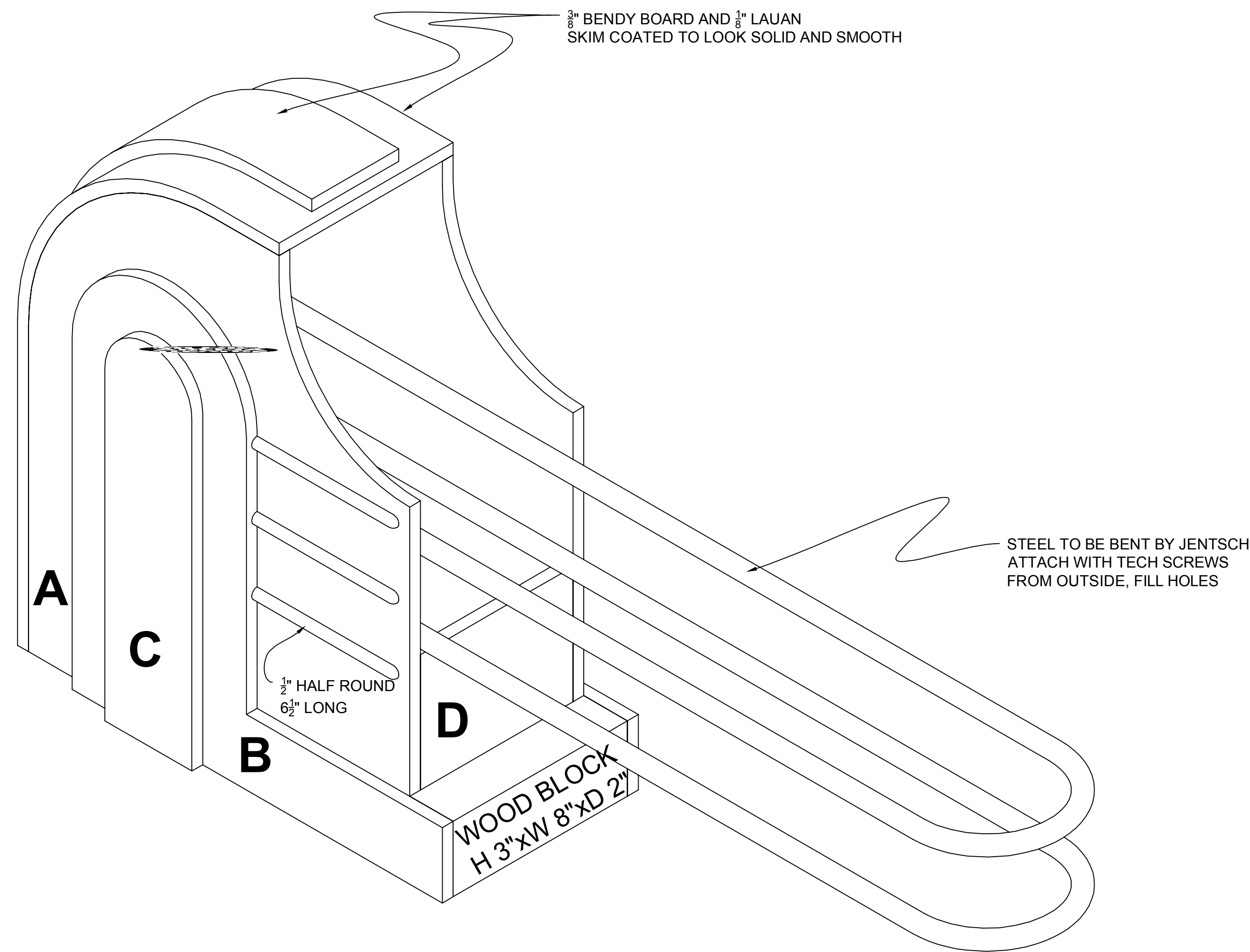
ISOMETRIC VIEW
