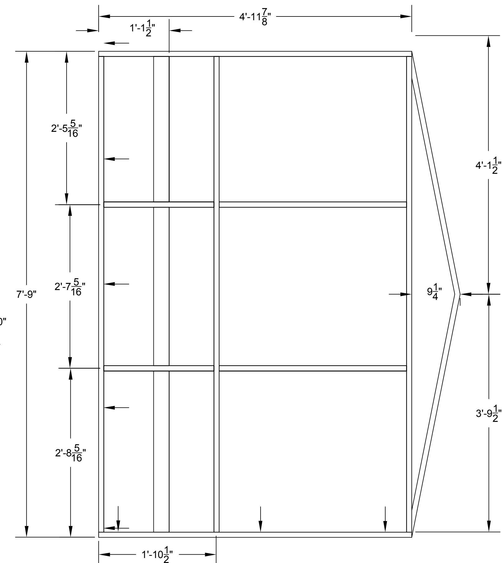
HOUSE WAGON FRAMING PLATFORM E
